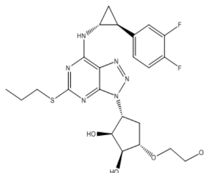
(1S,2S,3R,5S)-3-[7-[[[(1R,2S)-2-(3,4-difluorophenyl)cyclopropyl]amino]-5-propylsulfanyl]triazolo[5,4-d]pyrimidin-3-yl]-5-(2-hydroxyethoxy)cyclopentane-1,2-diol
